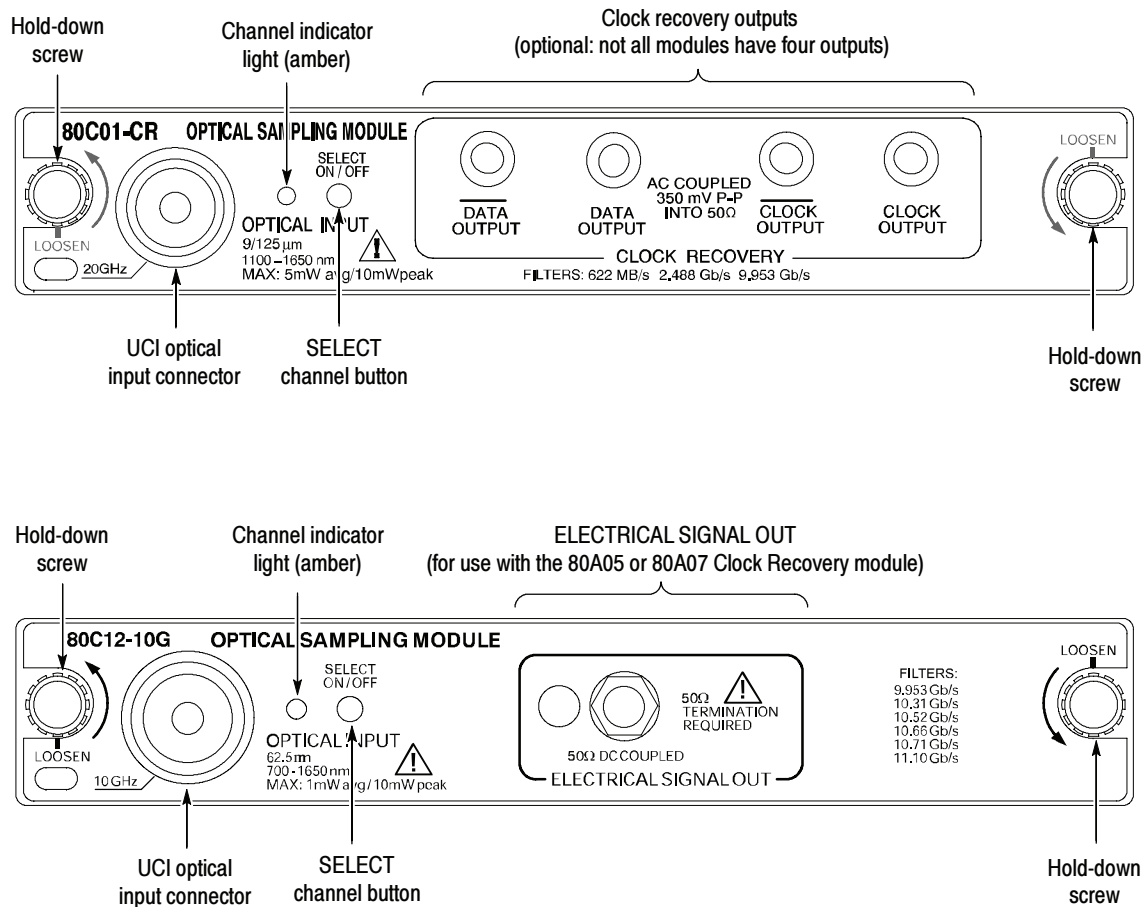
Figure 5: Typical Optical module front panels, 80C01-CR and 80C12 shown
